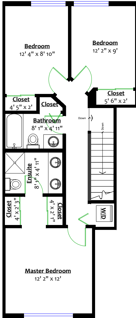
UPPER LEVEL Floor Area: 710 Sq. Ft.
